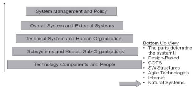
Figure 1: Multi-layered System
