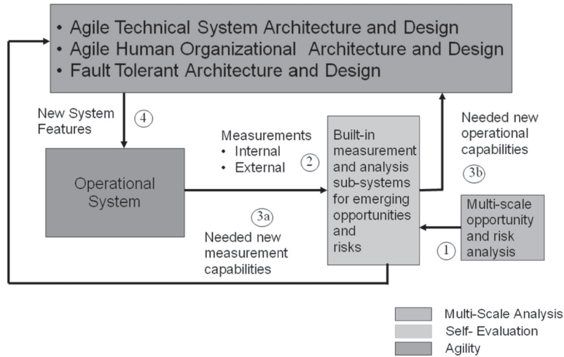
Figure 4: Design Framework for Agile Large-Scale Systems [Horowitz, 2007]
